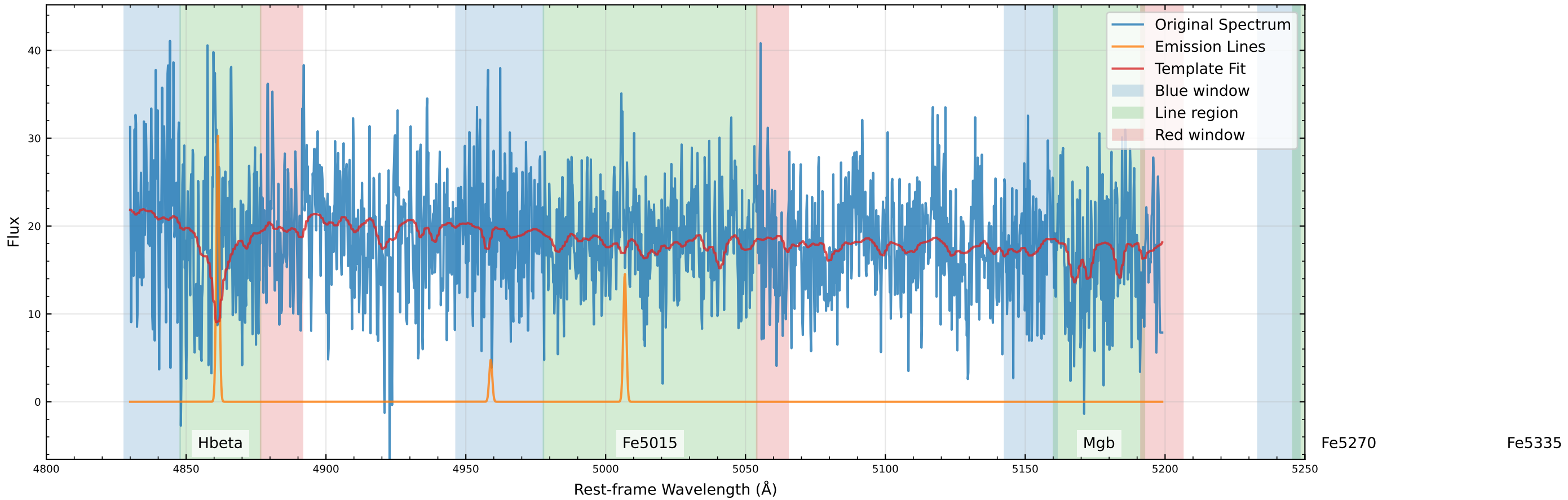
Original Data Comparison (v_star=-85.9 km/s, v_gas=-71.8 km/s)
