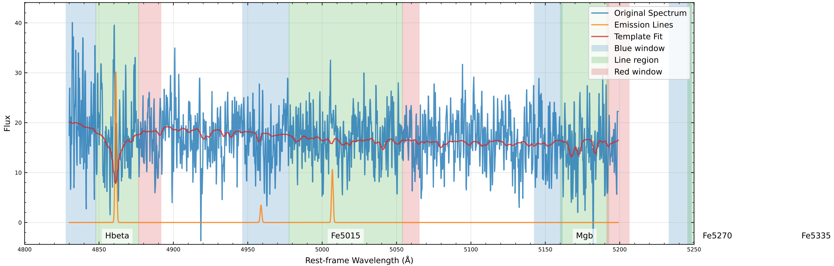
Original Data Comparison (v_star=-75.1 km/s, v_gas=-78.0 km/s)
