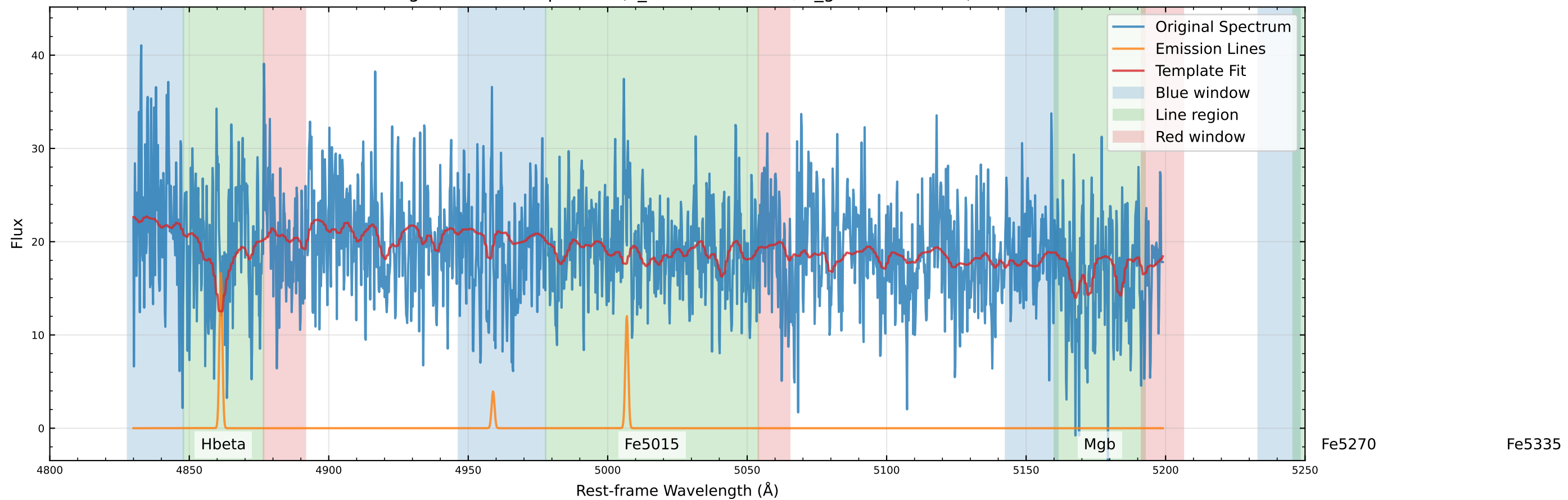
Original Data Comparison (v_star=-46.6 km/s, v_gas=-61.7 km/s)
