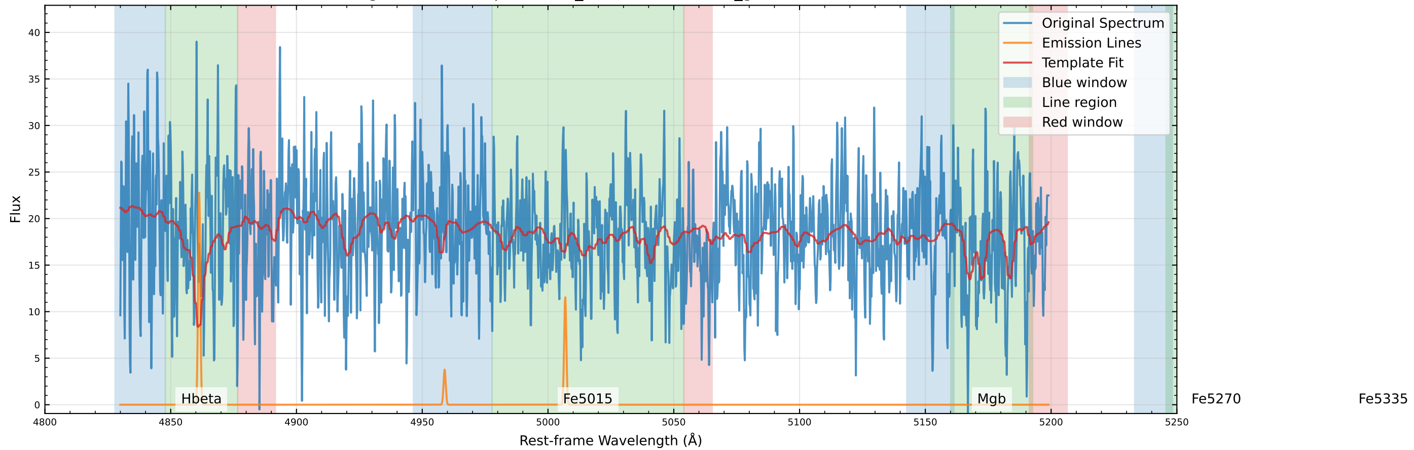
Original Data Comparison (v_star=-80.6 km/s, v_gas=-65.2 km/s)
