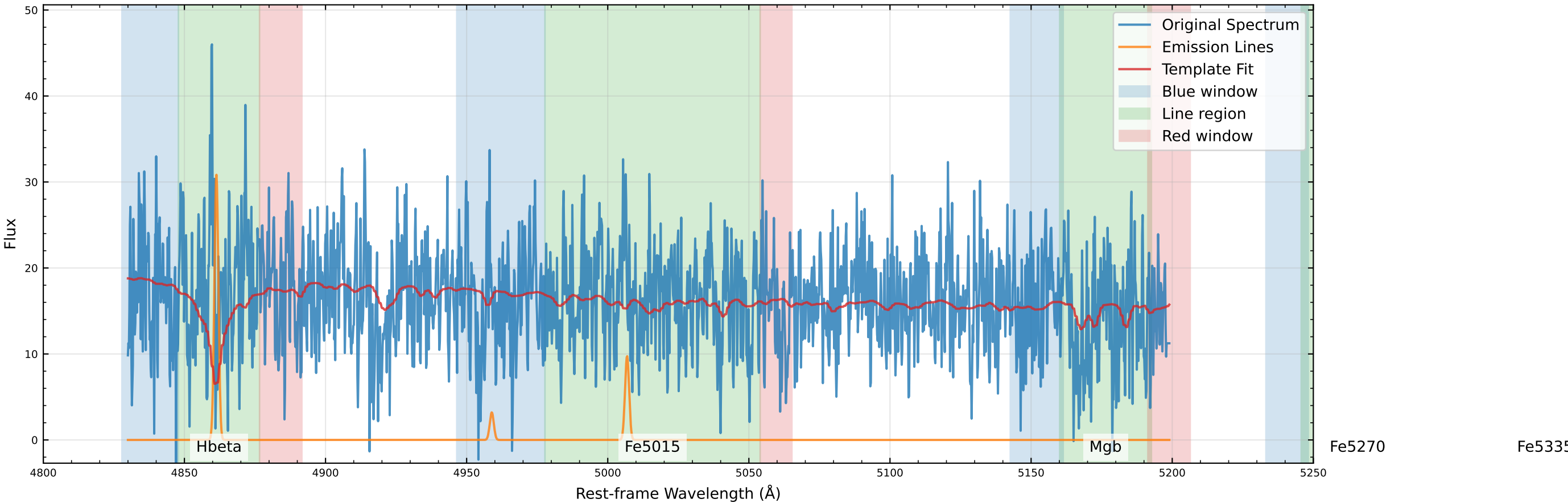
Original Data Comparison (v_star=-109.7 km/s, v_gas=-102.9 km/s)
