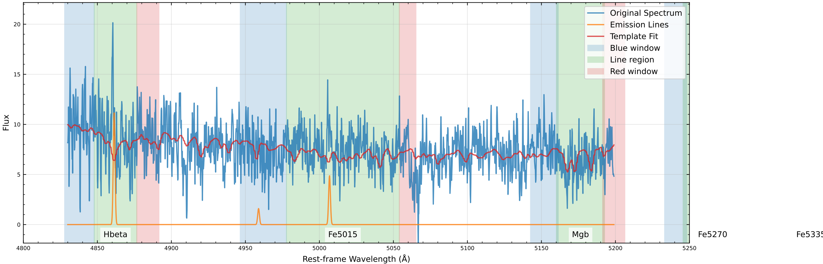
Original Data Comparison (v_star=-55.2 km/s, v_gas=-63.2 km/s)
