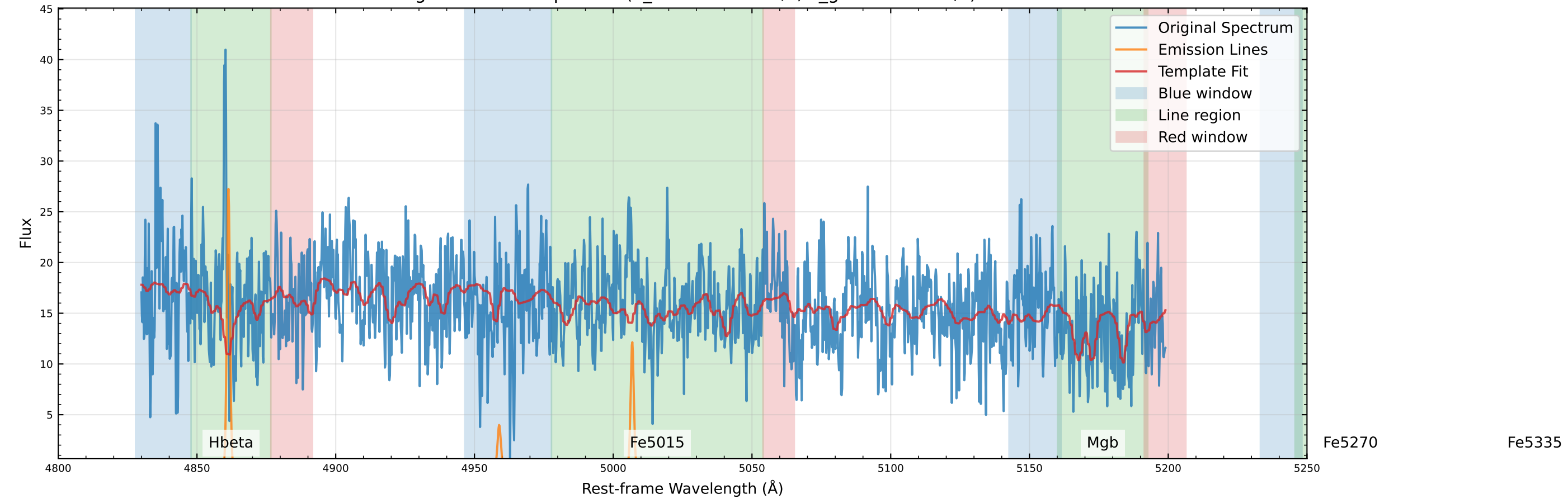
Original Data Comparison (v_star=-54.0 km/s, v_gas=-77.0 km/s)
