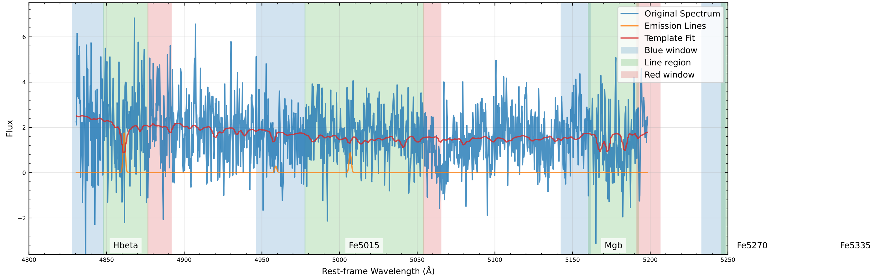
Original Data Comparison (v_star=71.6 km/s, v_gas=96.1 km/s)
