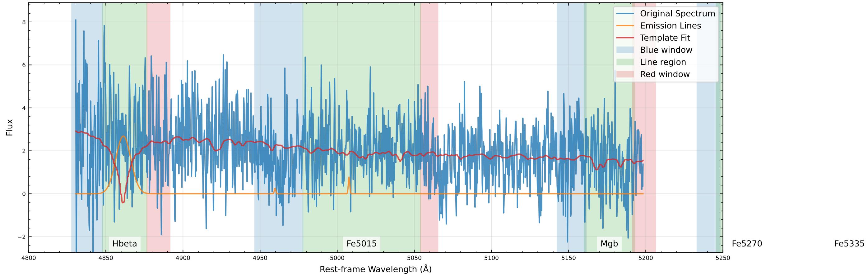
Original Data Comparison (v_star=-333.2 km/s, v_gas=-387.3 km/s)
