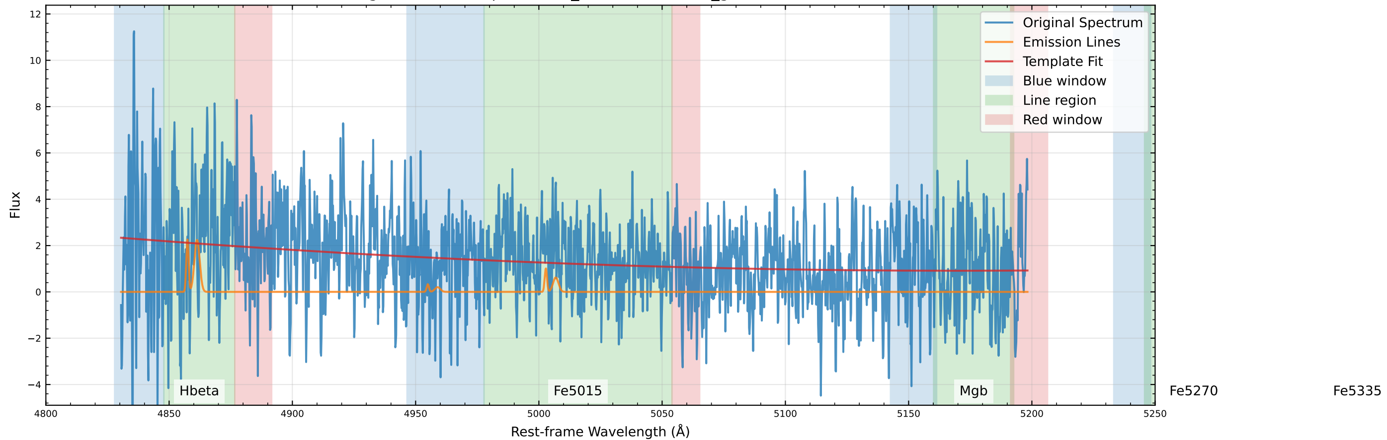
Original Data Comparison (v_star=0.0 km/s, v_gas=202.5 km/s)
