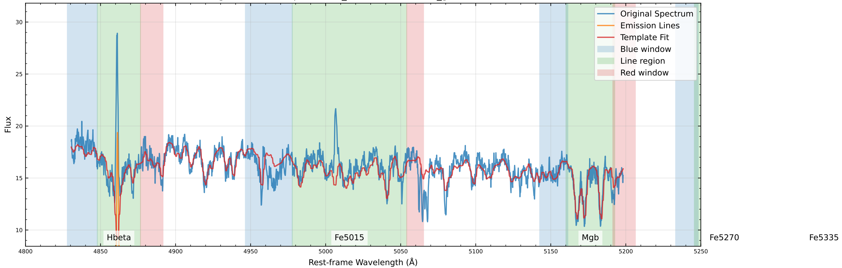
Original Data Comparison (v_star=-16.3 km/s, v_gas=-22.0 km/s)
