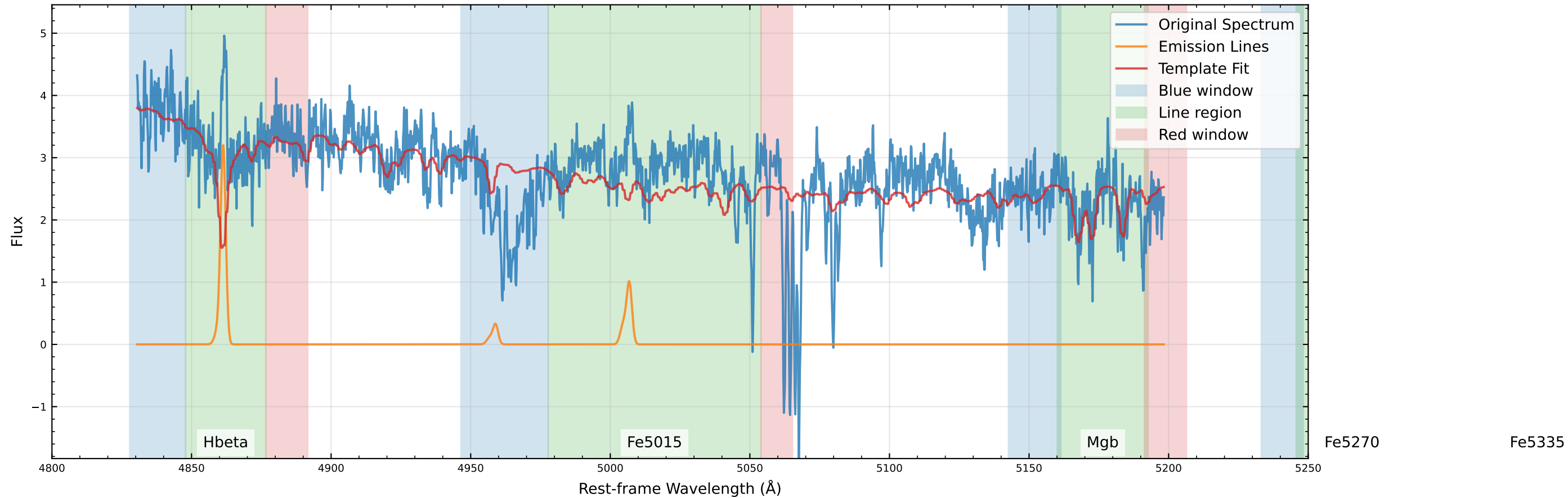
Original Data Comparison (v_star=-8.0 km/s, v_gas=12.0 km/s)
