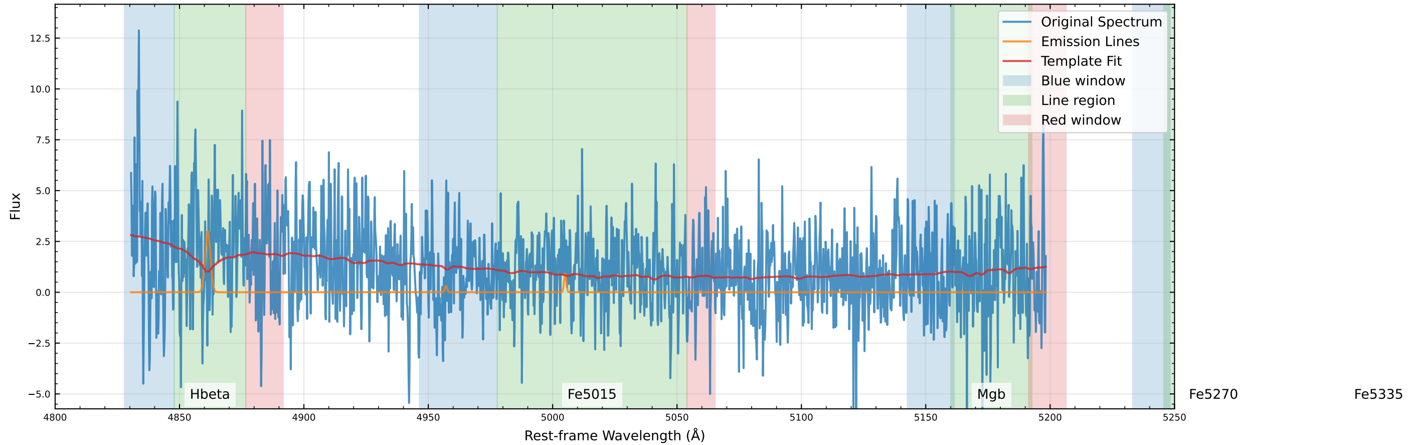
Original Data Comparison (v_star=-389.9 km/s, v_gas=-306.4 km/s)
