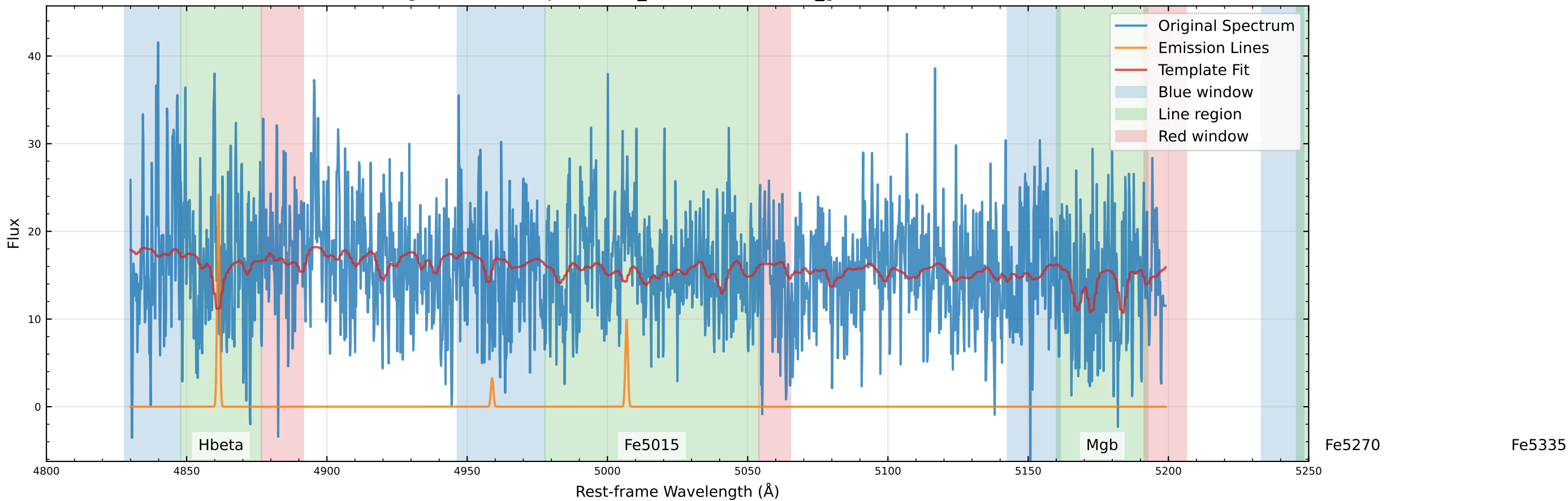
Original Data Comparison (v_star=-86.6 km/s, v_gas=-91.7 km/s)
