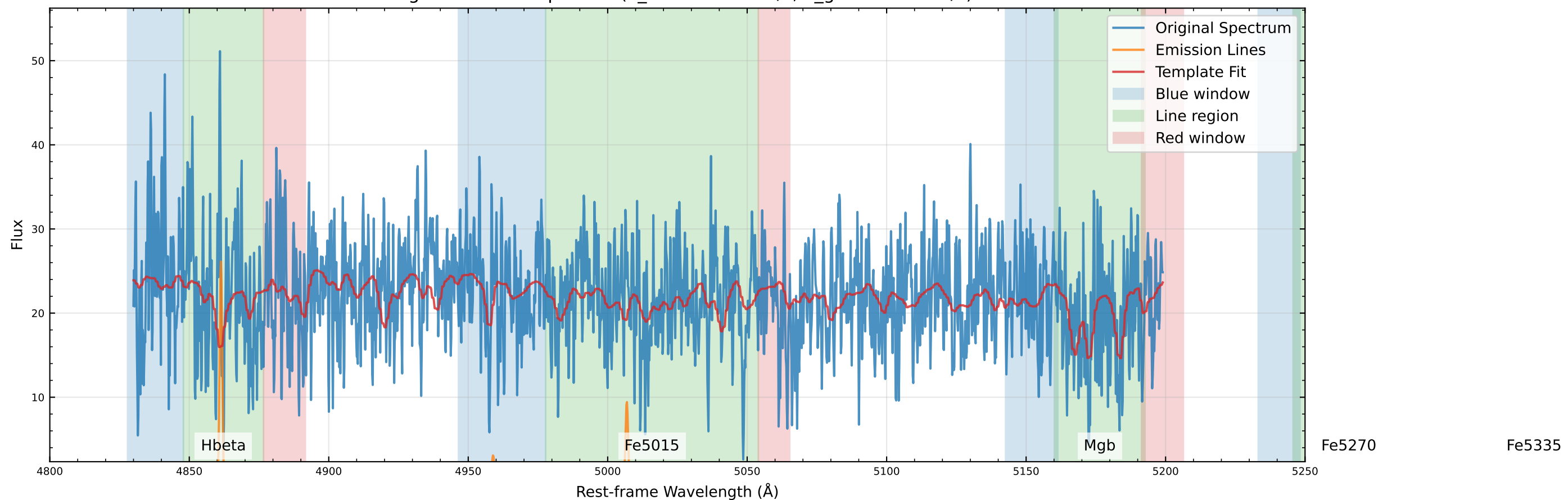
Original Data Comparison (v_star=-26.0 km/s, v_gas=-27.1 km/s)
