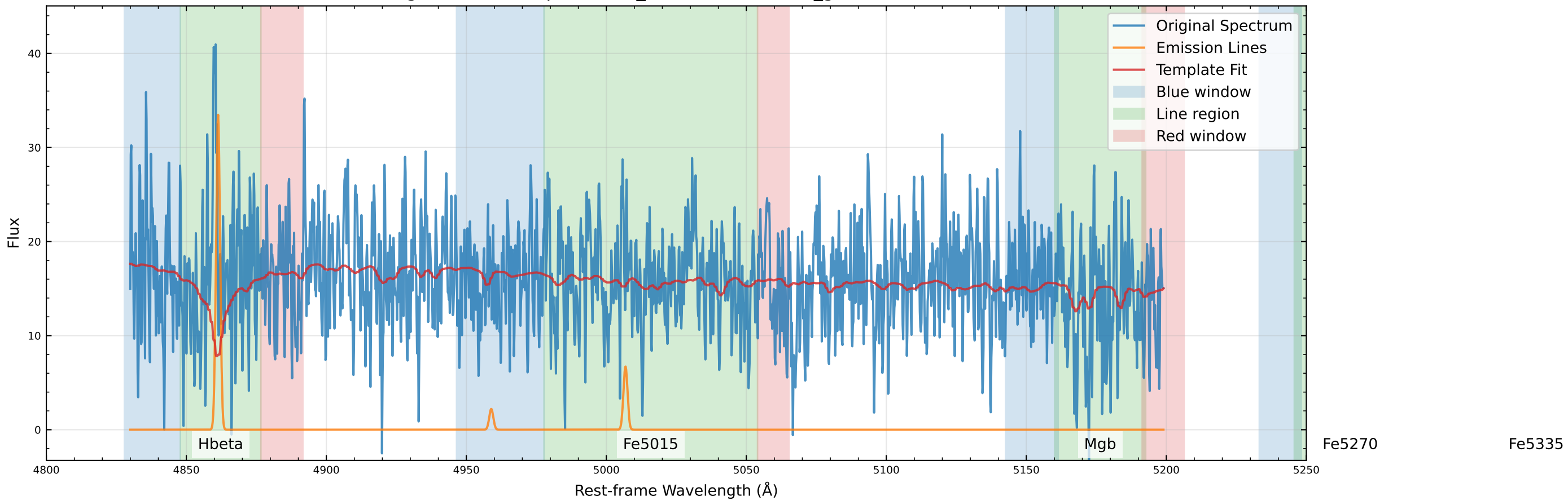
Original Data Comparison (v_star=-49.0 km/s, v_gas=-72.3 km/s)
