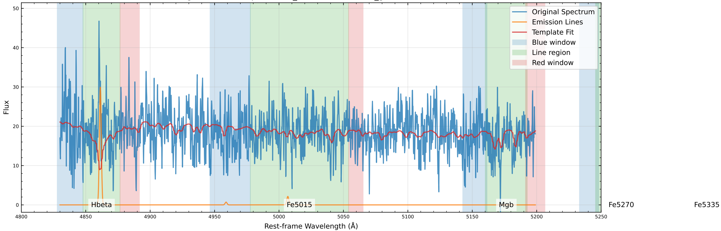
Original Data Comparison (v_star=-49.2 km/s, v_gas=-52.3 km/s)
