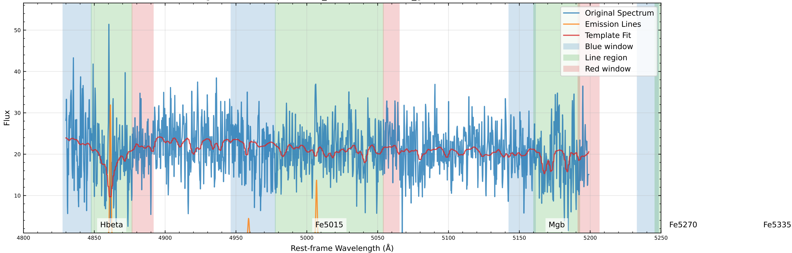
Original Data Comparison (v_star=-75.2 km/s, v_gas=-61.7 km/s)
