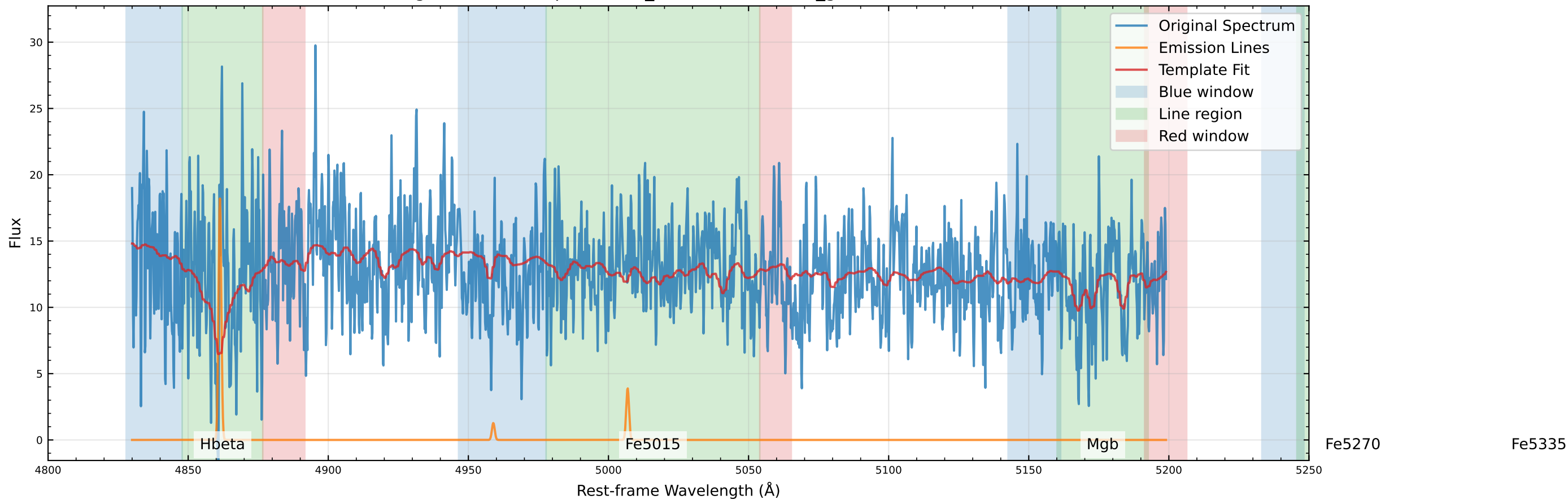
Original Data Comparison (v_star=26.2 km/s, v_gas=40.2 km/s)
