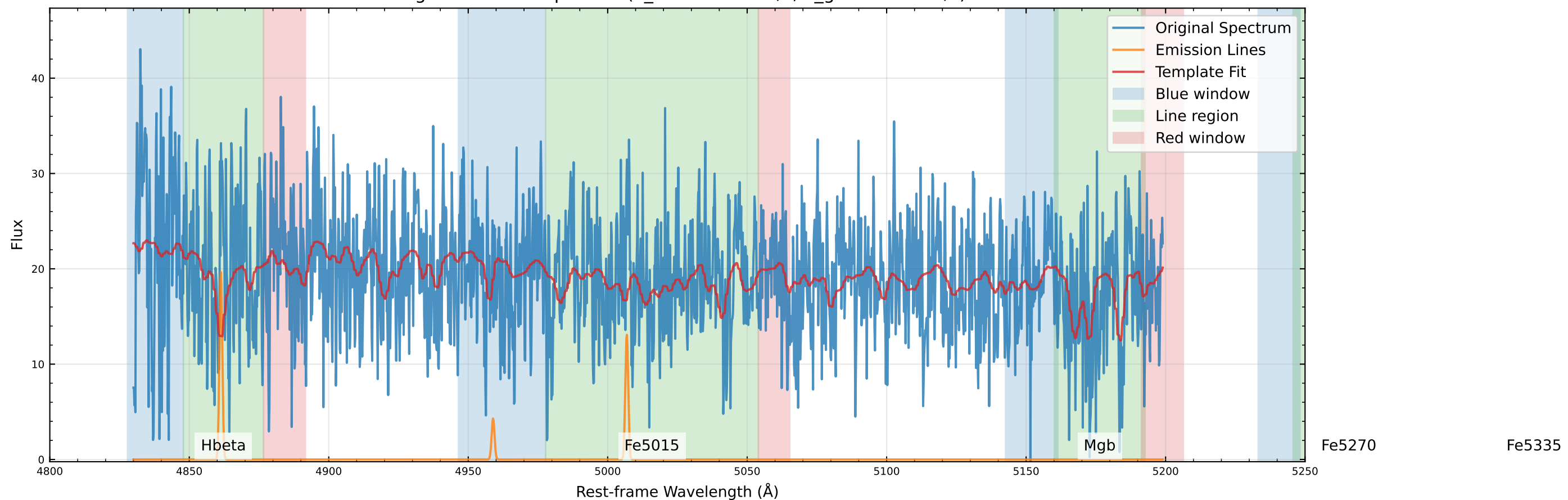
Original Data Comparison (v_star=22.6 km/s, v_gas=20.1 km/s)
