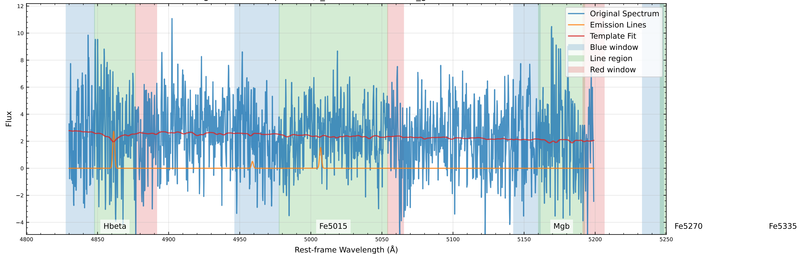
Original Data Comparison (v_star=-186.5 km/s, v_gas=-264.9 km/s)
