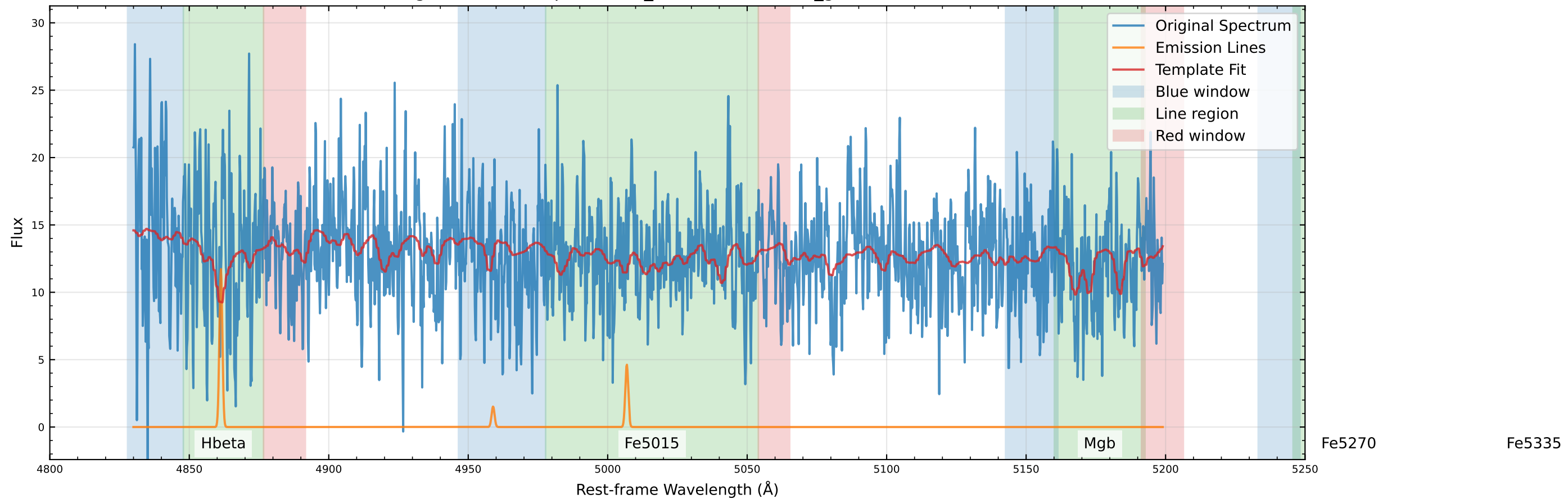
Original Data Comparison (v_star=40.0 km/s, v_gas=57.2 km/s)
