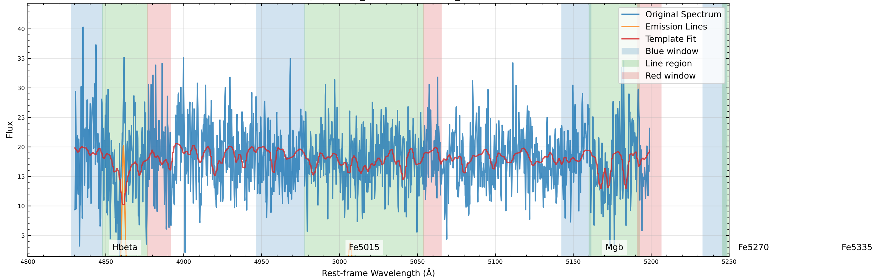
Original Data Comparison (v_star=58.7 km/s, v_gas=26.5 km/s)
