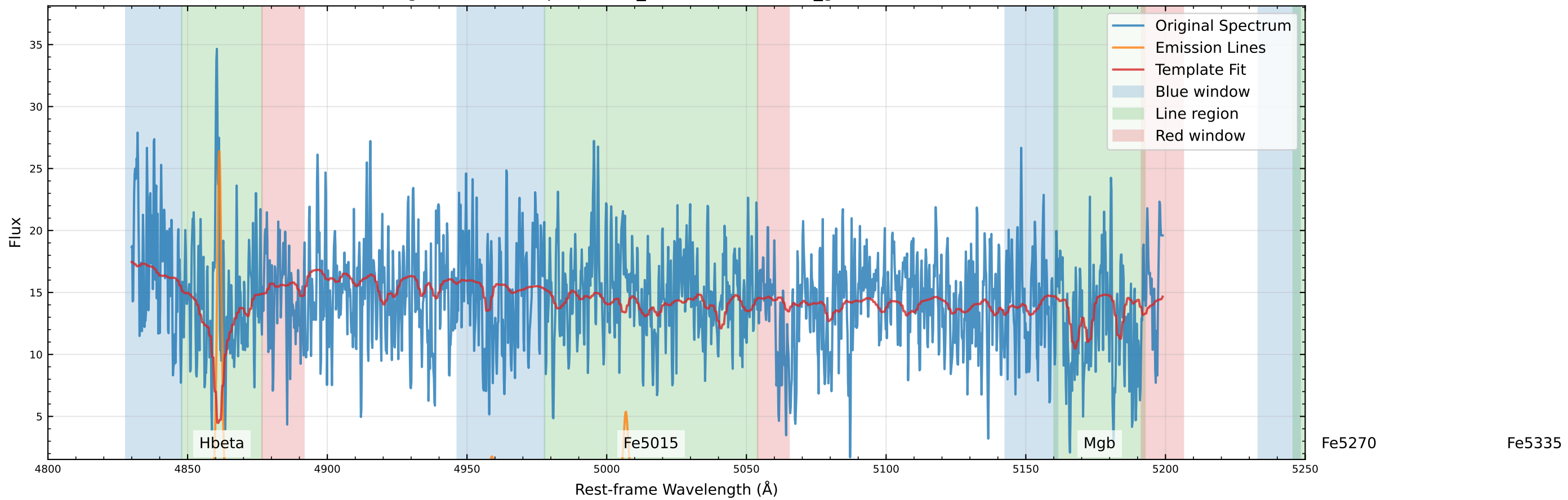
Original Data Comparison (v_star=-87.3 km/s, v_gas=-58.1 km/s)
