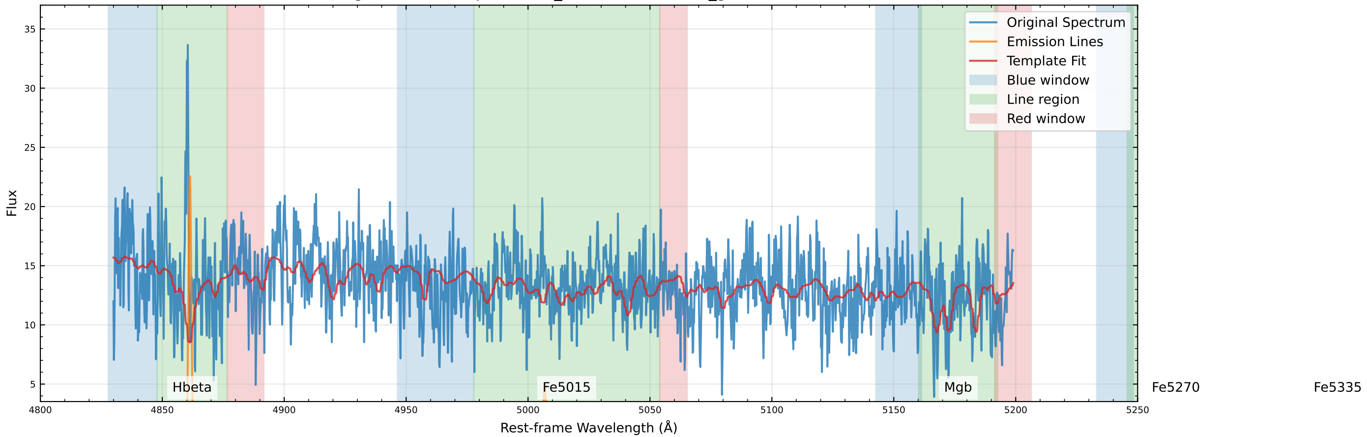
Original Data Comparison (v_star=-57.0 km/s, v_gas=-72.2 km/s)
