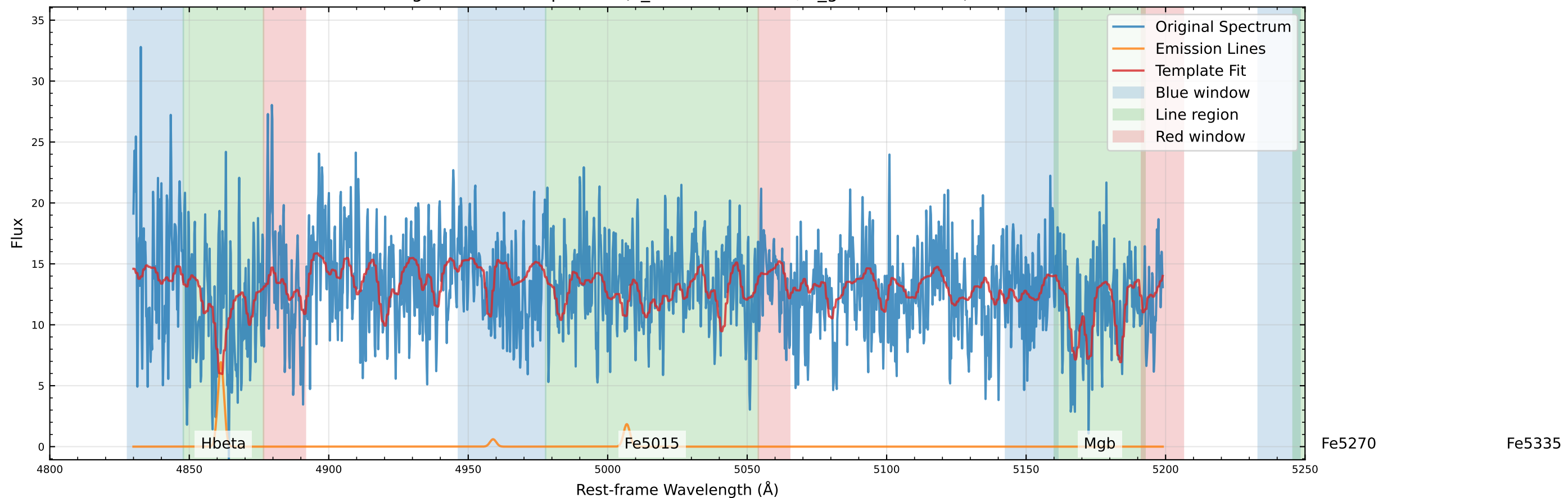
Original Data Comparison (v_star=-24.9 km/s, v_gas=18.3 km/s)
