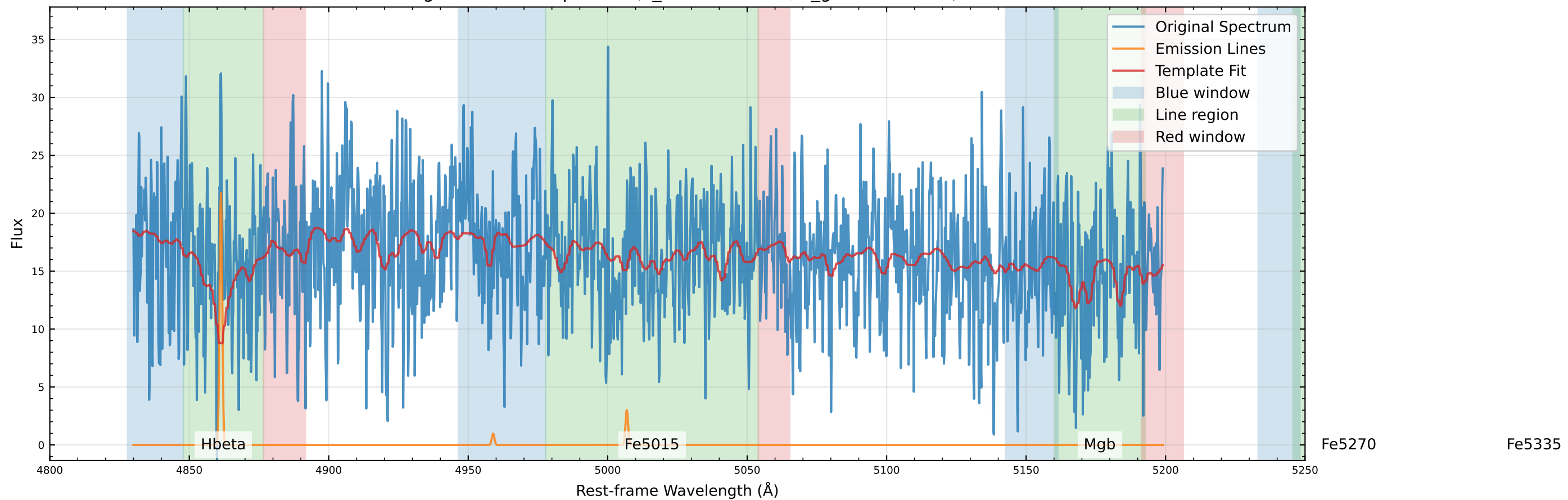
Original Data Comparison (v_star=5.1 km/s, v_gas=-1.1 km/s)
