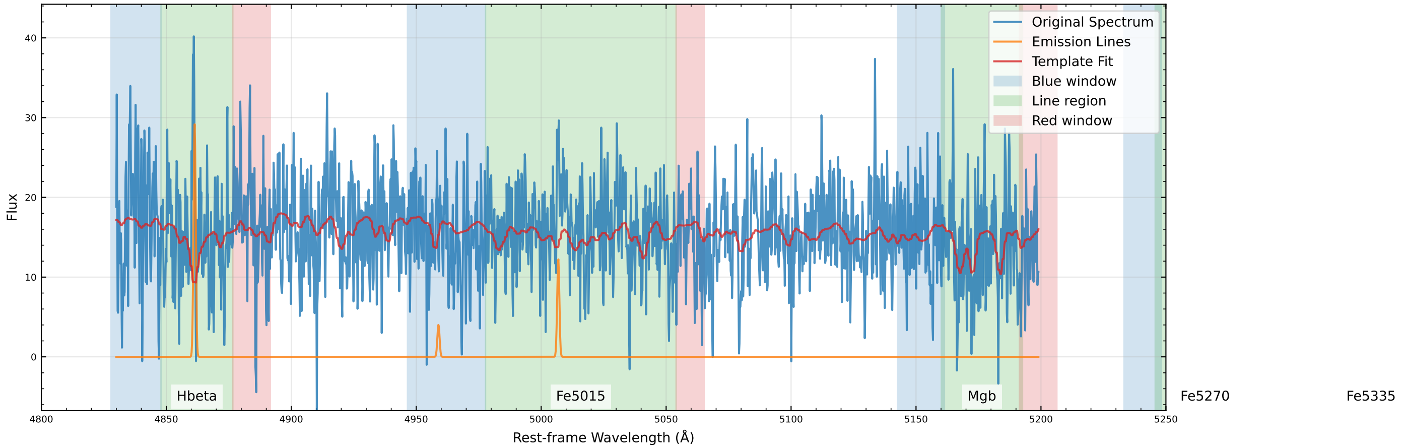
Original Data Comparison (v_star=-17.1 km/s, v_gas=-26.2 km/s)
