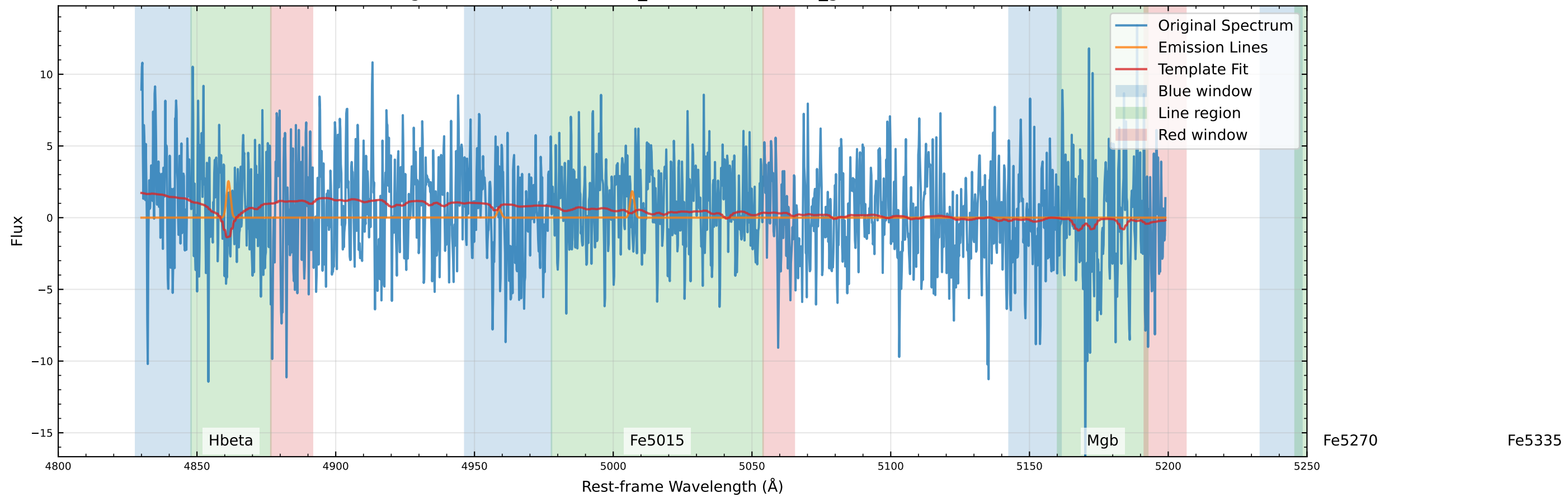
Original Data Comparison (v_star=121.8 km/s, v_gas=120.5 km/s)
