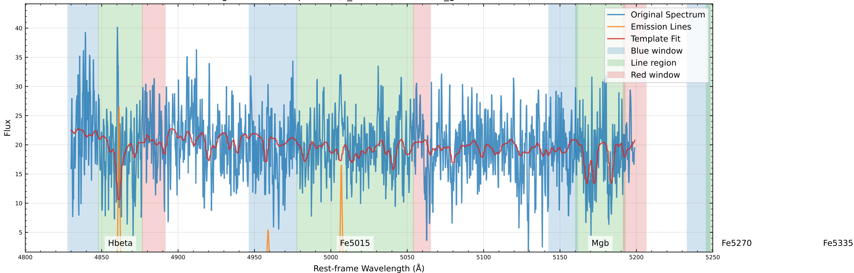
Original Data Comparison (v_star=-37.9 km/s, v_gas=-48.1 km/s)
