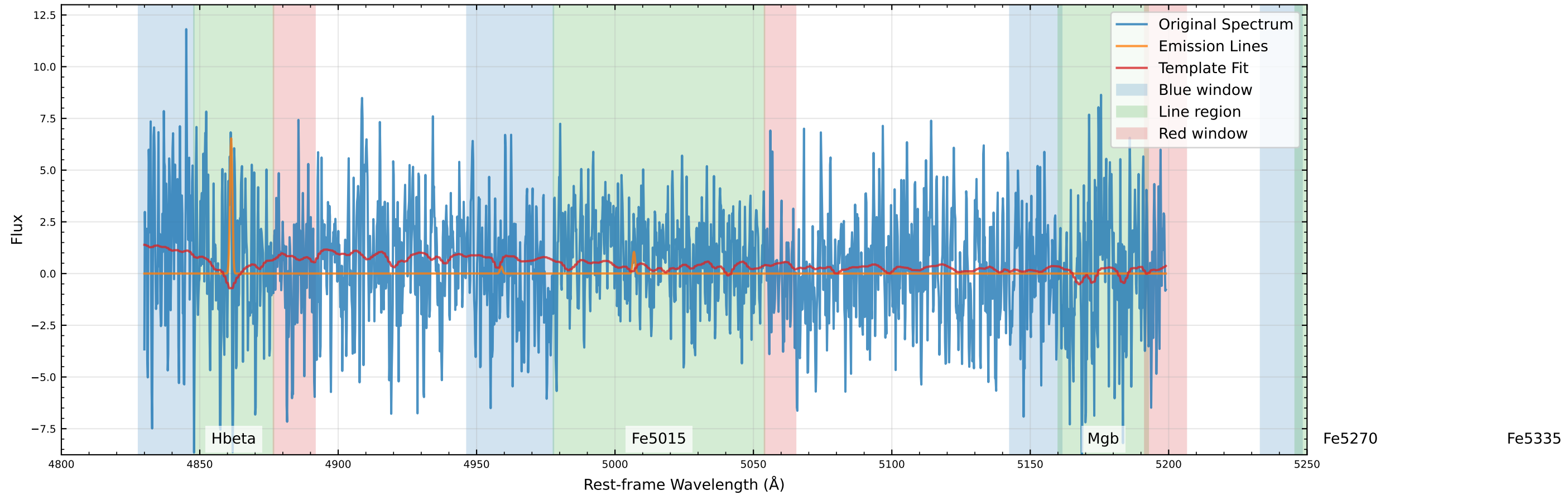
Original Data Comparison (v_star=-20.4 km/s, v_gas=-28.0 km/s)
