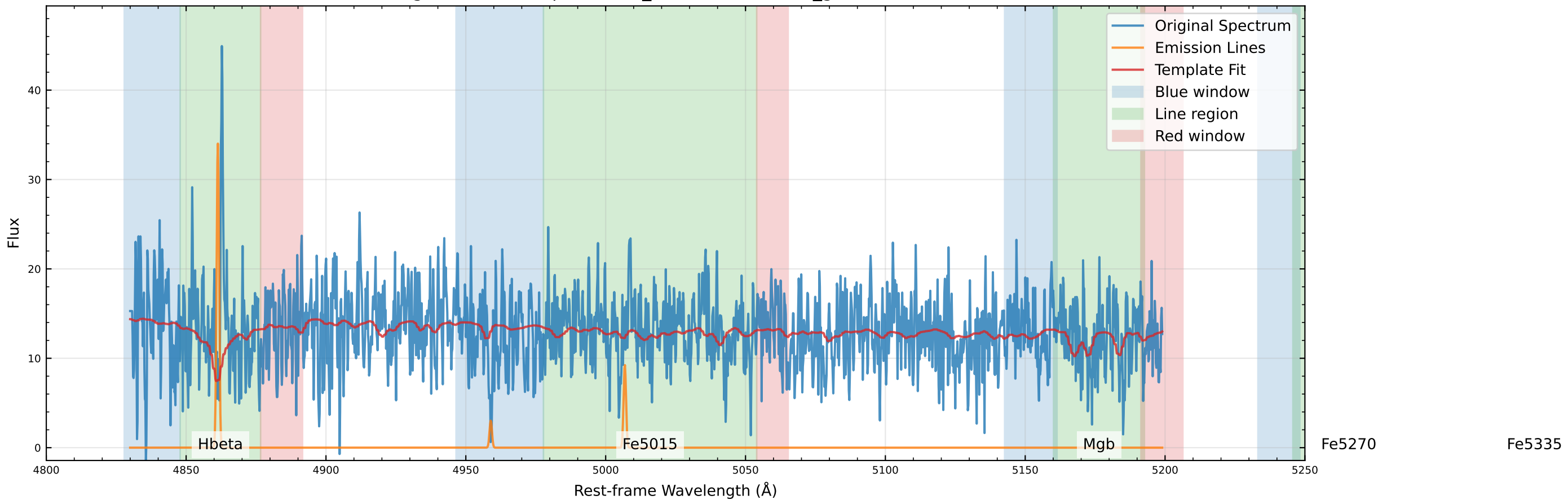
Original Data Comparison (v_star=91.5 km/s, v_gas=93.8 km/s)
