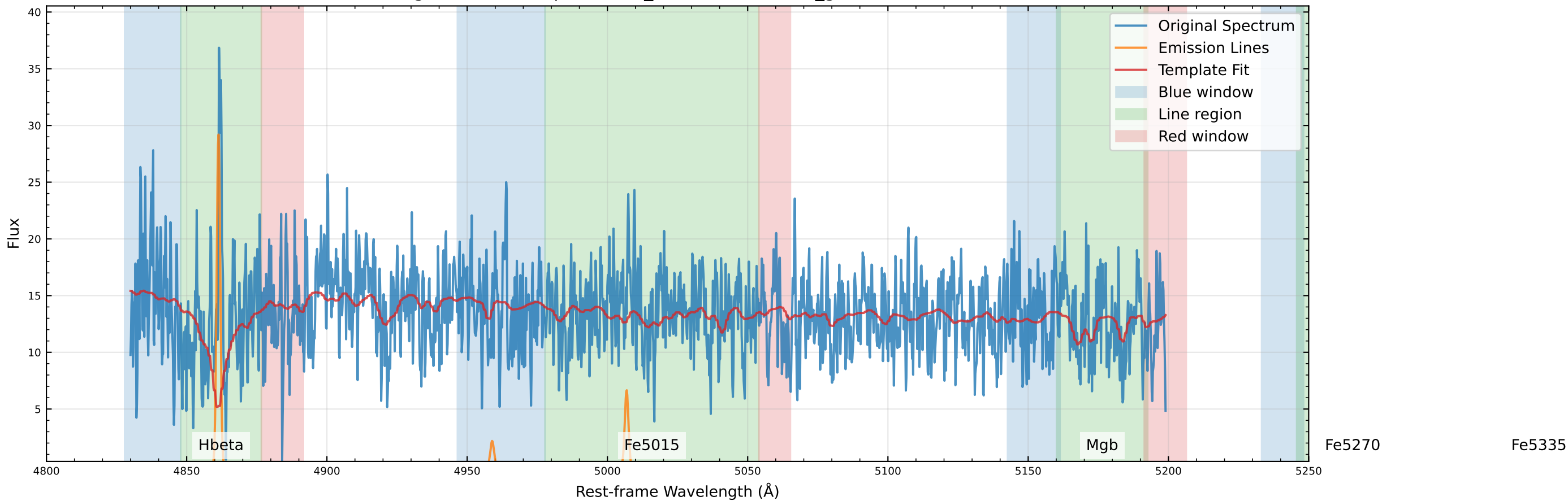
Original Data Comparison (v_star=10.5 km/s, v_gas=35.6 km/s)
