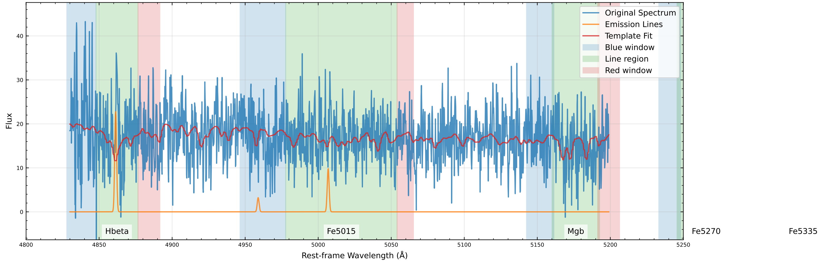
Original Data Comparison (v_star=43.3 km/s, v_gas=53.6 km/s)
