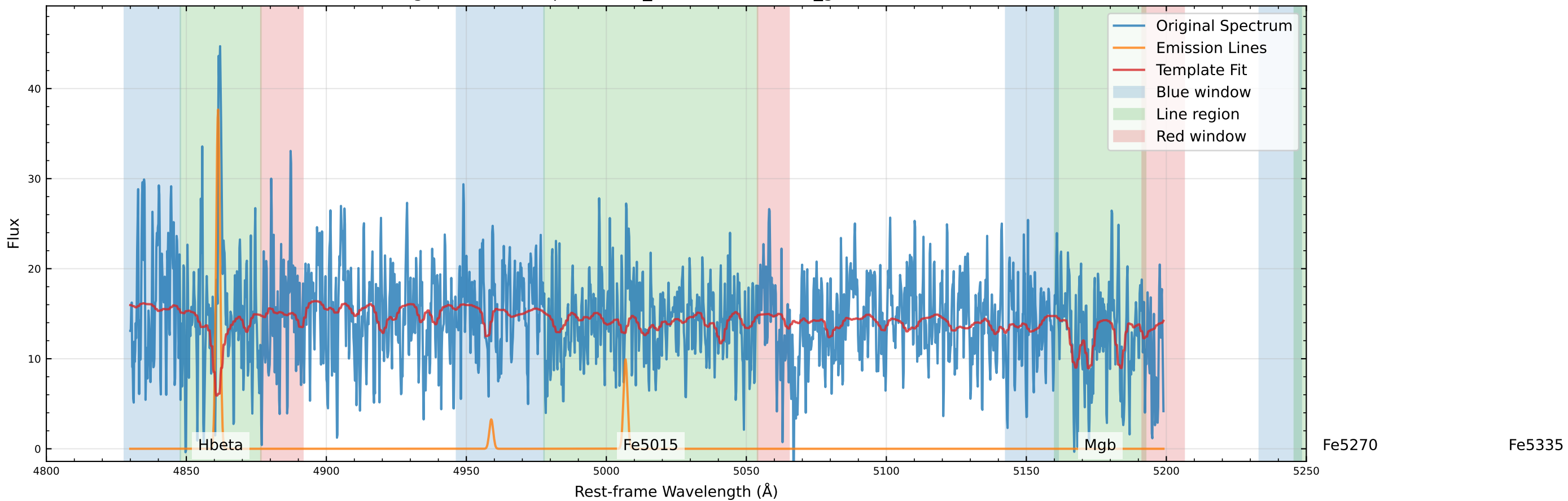
Original Data Comparison ( v_{\text{star}}=36.7 km/s, v_{\text{gas}}=41.2 km/s)
