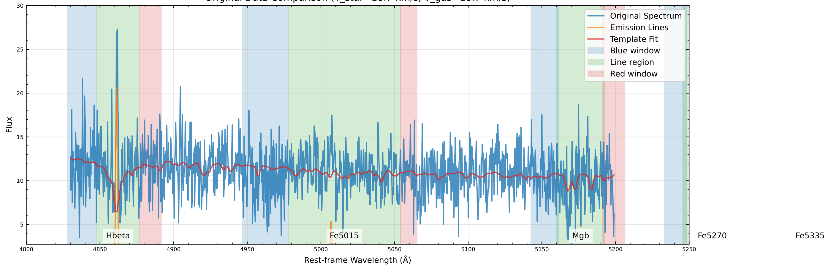
Original Data Comparison (v_star=18.7 km/s, v_gas=18.7 km/s)
