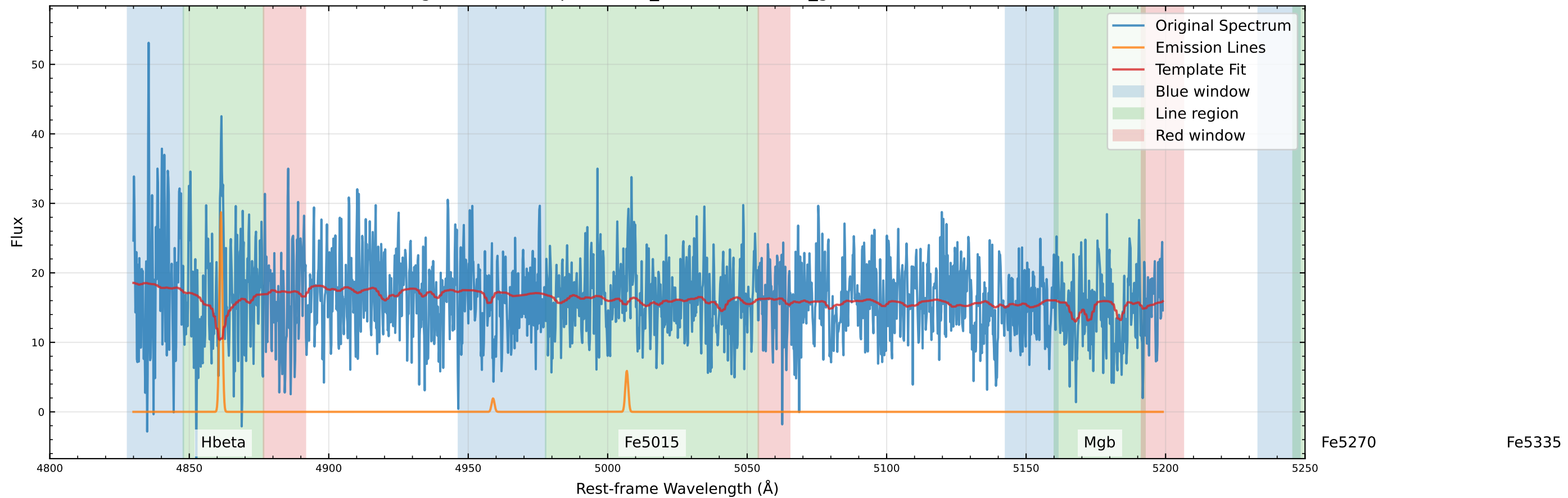
Original Data Comparison (v_star=6.4 km/s, v_gas=17.9 km/s)
