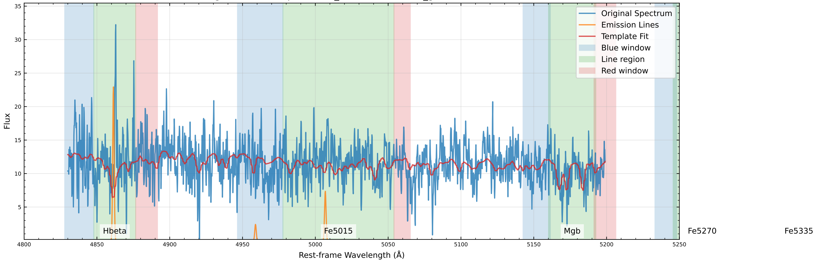
Original Data Comparison (v_star=75.9 km/s, v_gas=87.0 km/s)
