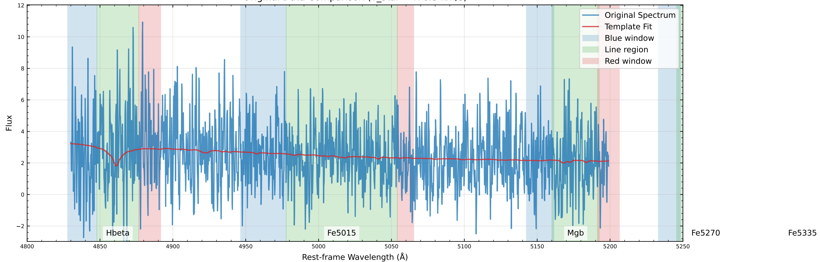
Original Data Comparison ( v_{\text{star}} = -476.3 km/s)
