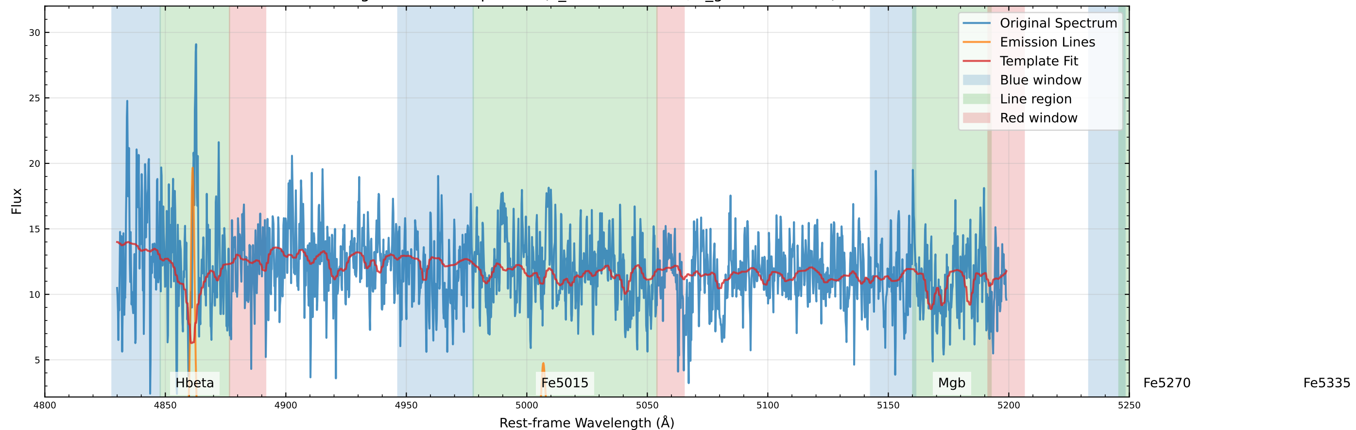
Original Data Comparison (v_star=67.7 km/s, v_gas=72.6 km/s)
