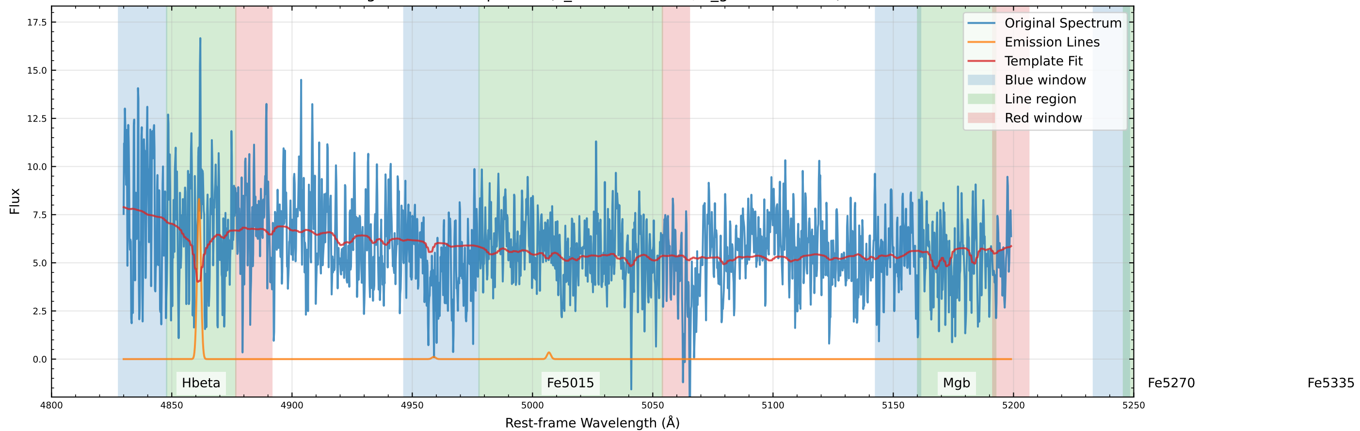
Original Data Comparison (v_star=13.3 km/s, v_gas=32.3 km/s)
