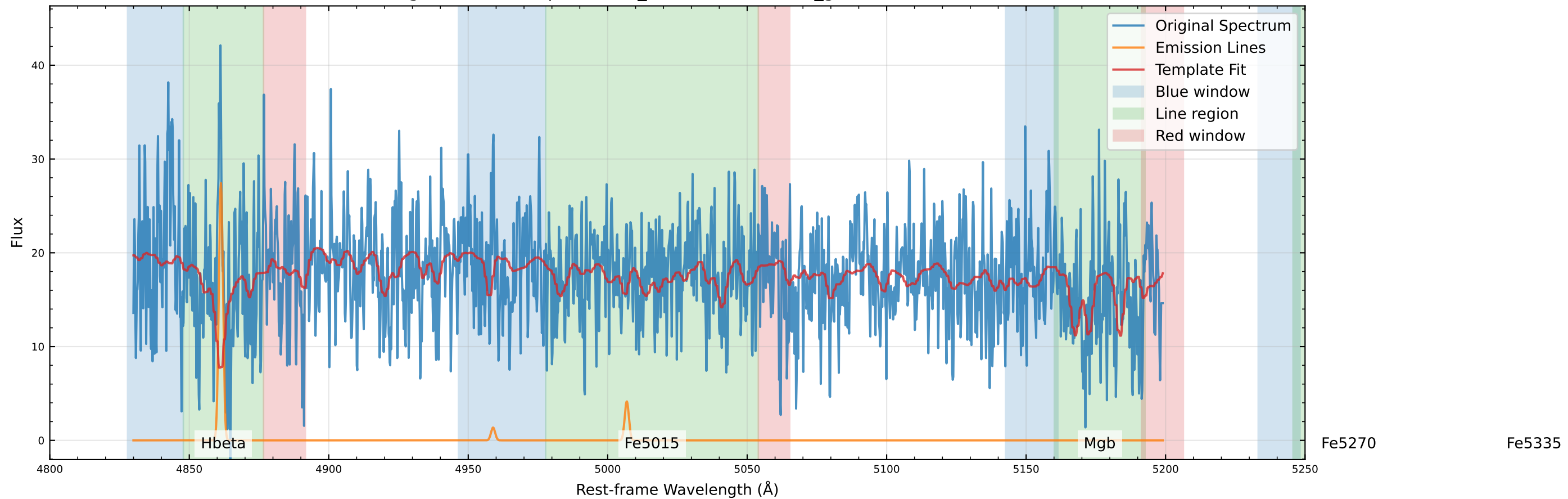
Original Data Comparison ( v_{\text{star}}=-68.7 km/s, v_{\text{gas}}=-28.3 km/s)
