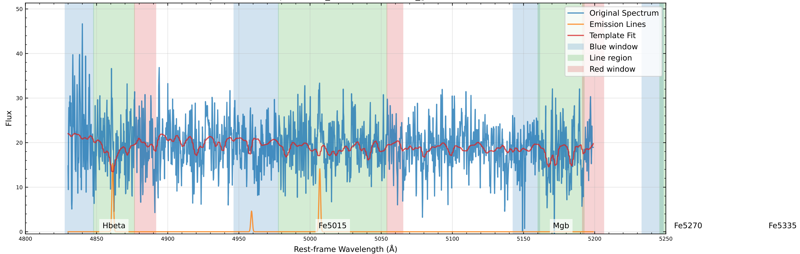
Original Data Comparison (v_star=-60.4 km/s, v_gas=-36.1 km/s)
