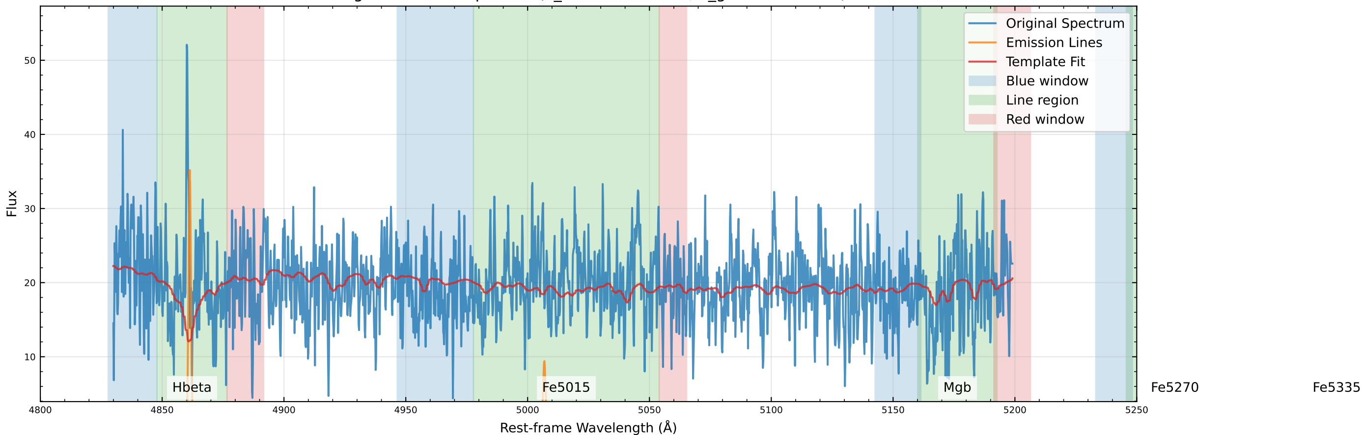
Original Data Comparison (v_star=-78.7 km/s, v_gas=-63.4 km/s)
