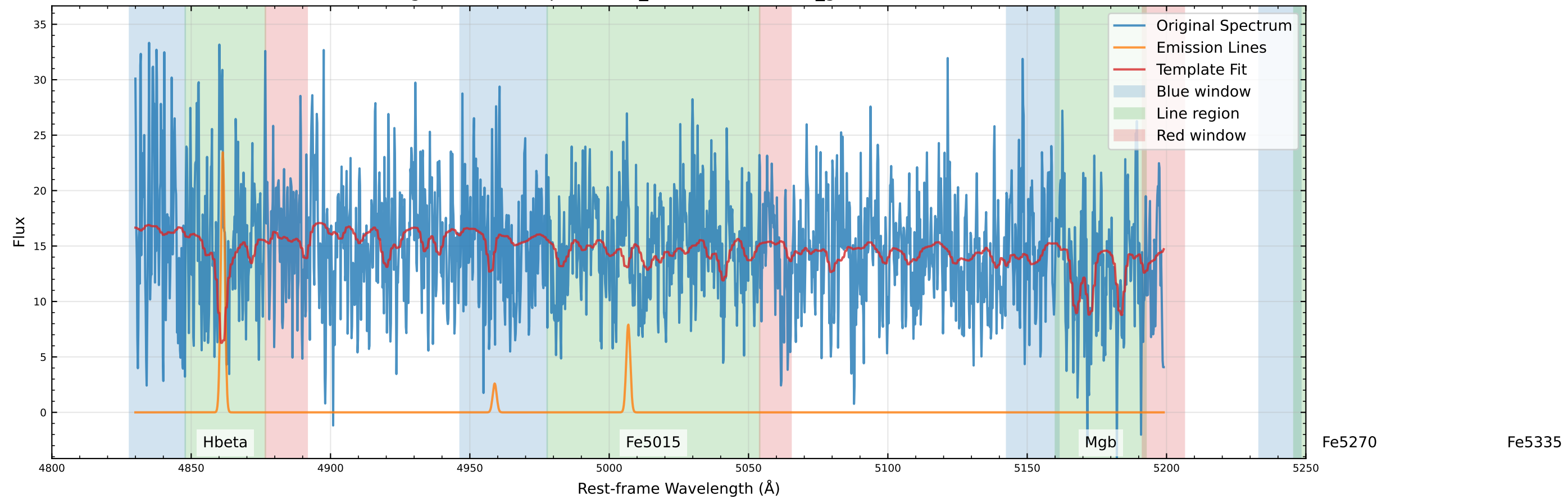
Original Data Comparison (v_star=-40.3 km/s, v_gas=-40.6 km/s)
