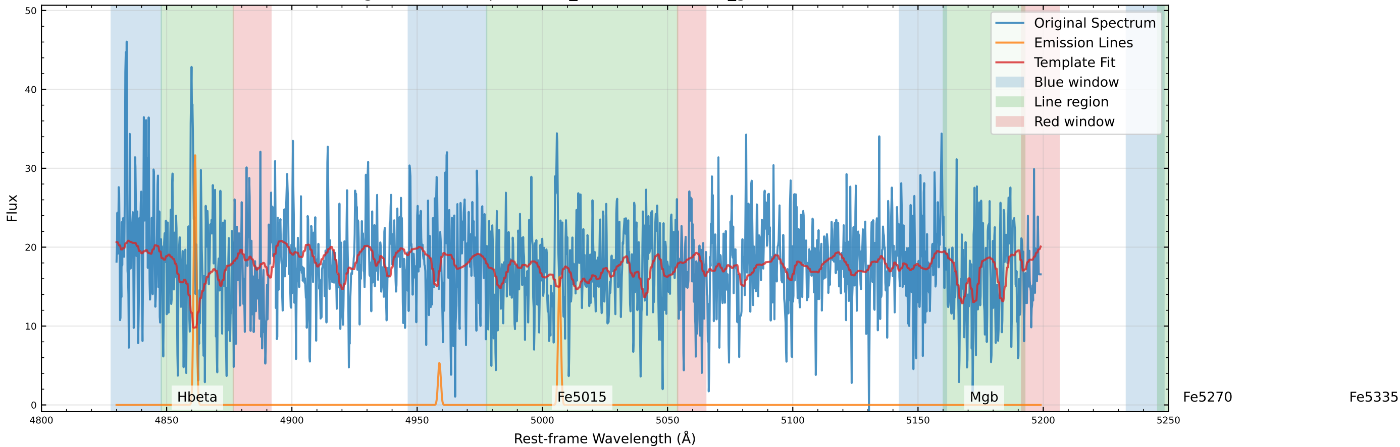
Original Data Comparison (v_star=-97.2 km/s, v_gas=-74.9 km/s)
