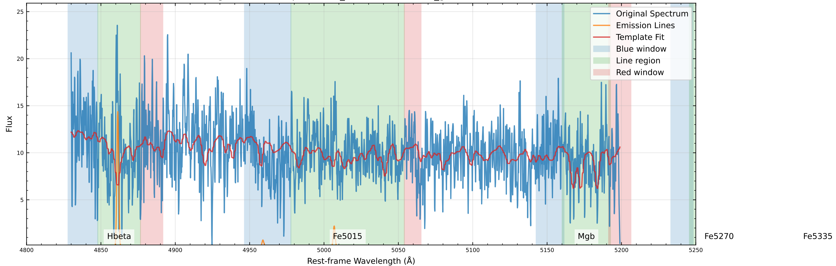
Original Data Comparison (v_star=-26.1 km/s, v_gas=-37.5 km/s)
