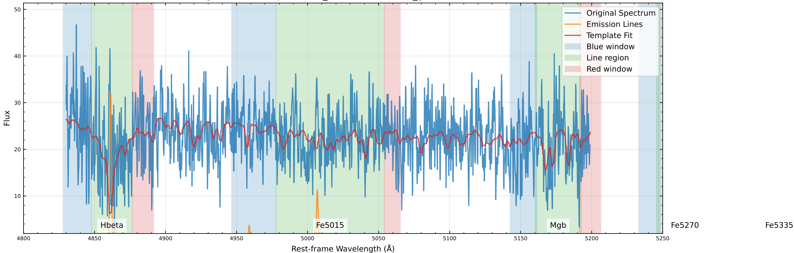
Original Data Comparison (v_star=-34.4 km/s, v_gas=-44.4 km/s)
