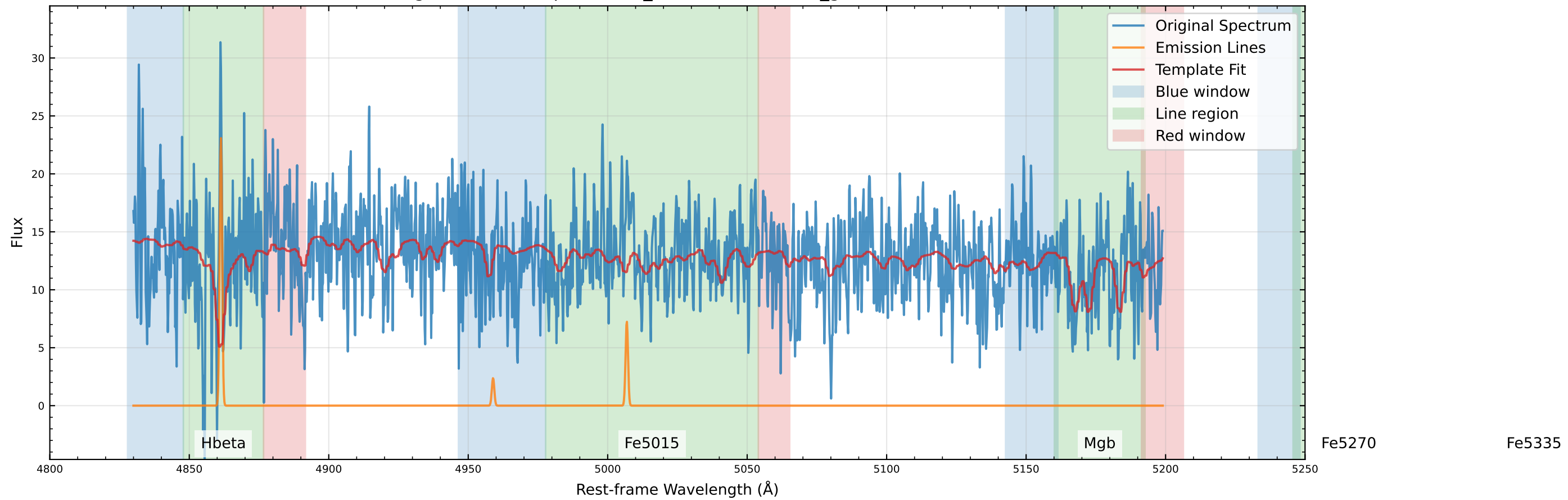
Original Data Comparison (v_star=-24.9 km/s, v_gas=-7.0 km/s)
