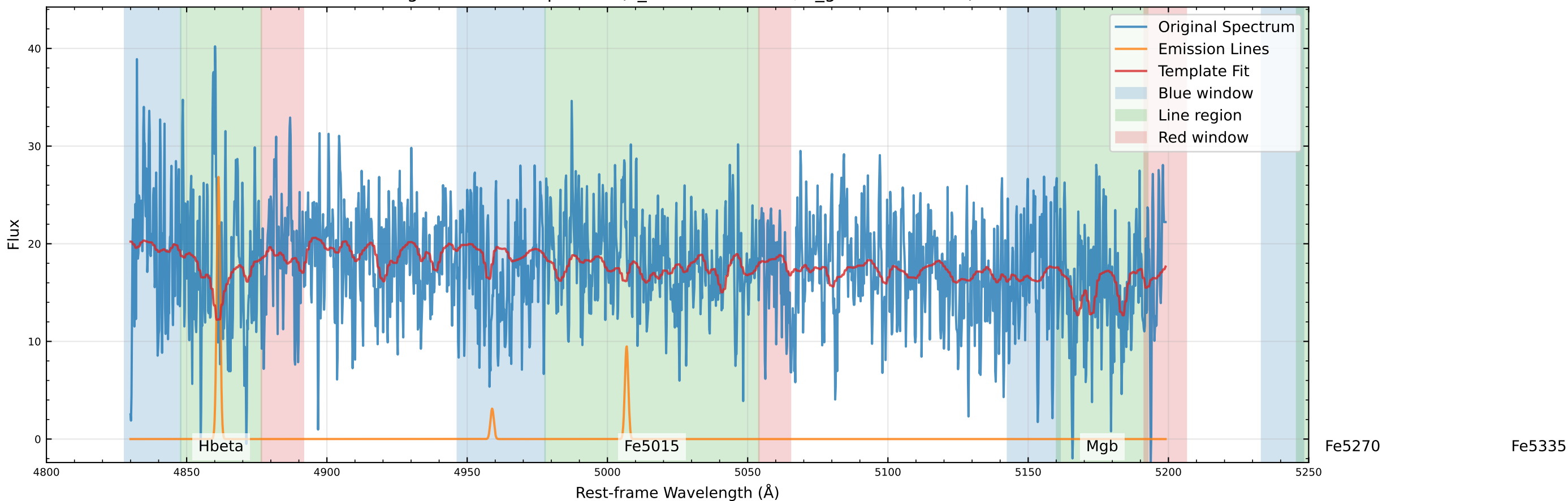
Original Data Comparison (v_star=-82.5 km/s, v_gas=-89.4 km/s)
